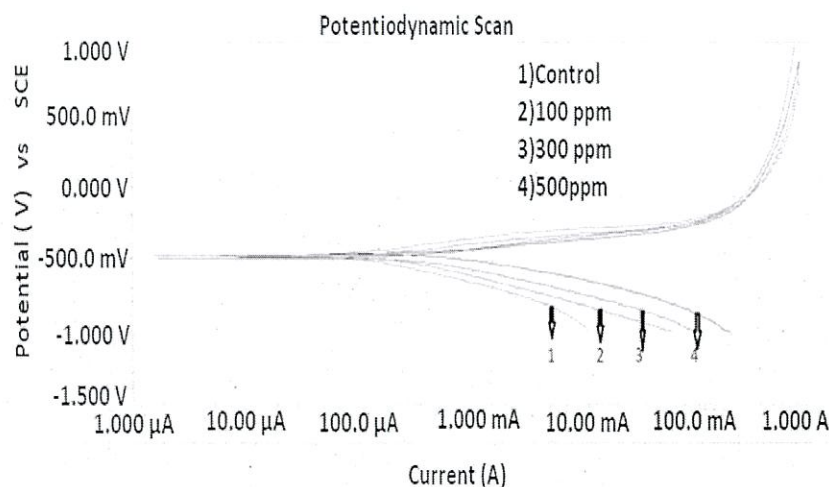
Fig. 5. Potentiodynamic polarization curves for mild steel without and with different concentrations of MIZ in Barr's medium inoculated with SRB.
