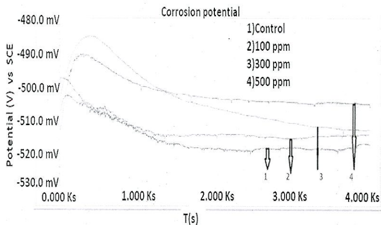
Fig. 3. Open circuit potential of mild steel without and with different concentrations of 2-methylimidazole (MIZ) in Barr's medium inoculated with SRB.
