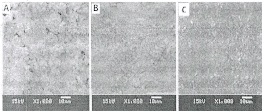
Fig. 6. SEM images of mild steel surface recovered from (A) Barr's medium inoculated with SRB (B) 500 ppm of MNZ (C) 500 ppm of MIZ.
