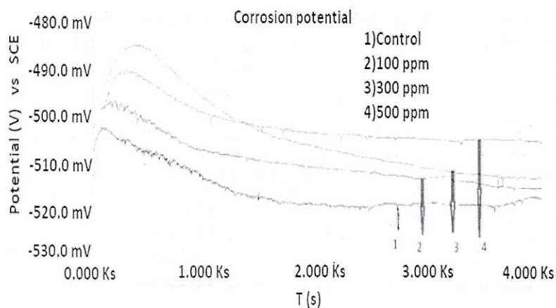
Fig. 2. Open circuit potential of mild steel without and with different concentrations of metronidazole (MNZ) in Barr's medium inoculated with SRB.
