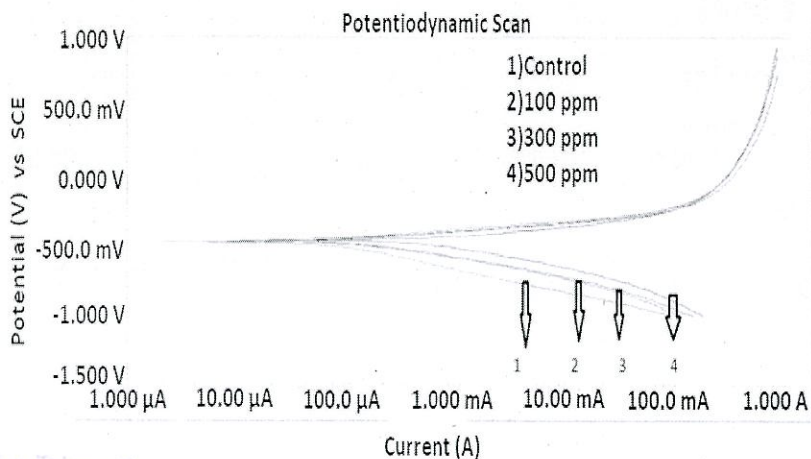
Fig. 4. Potentiodynamic polarization curves for mild steel without and with different concentrations of MNZ in Barr's medium inoculated with SRB.
