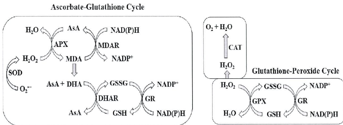
Fig. 3: Ascorbate-Glutathione Cycle and Glutathione-peroxidase Cycle
