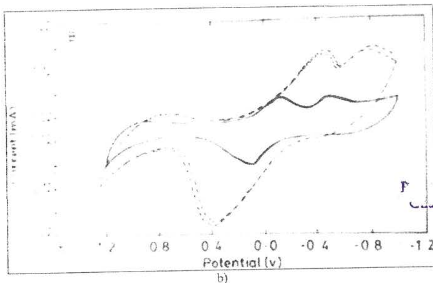
Fig 2: Cyclic voltammogram of Cu 2 O in DMSO (A) multicyclic, (B) beyond 1.2V
